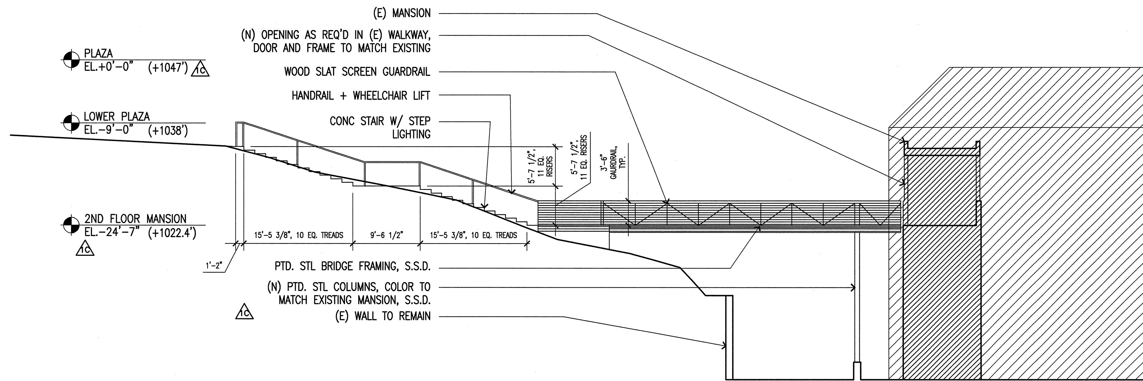
3 ELEVATION OF BRIDGE TO MANSION (ADD ALT. #1)
